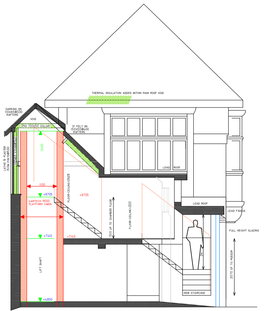
CROSS SECTION PROPOSED WITH LIFTSHAFT
