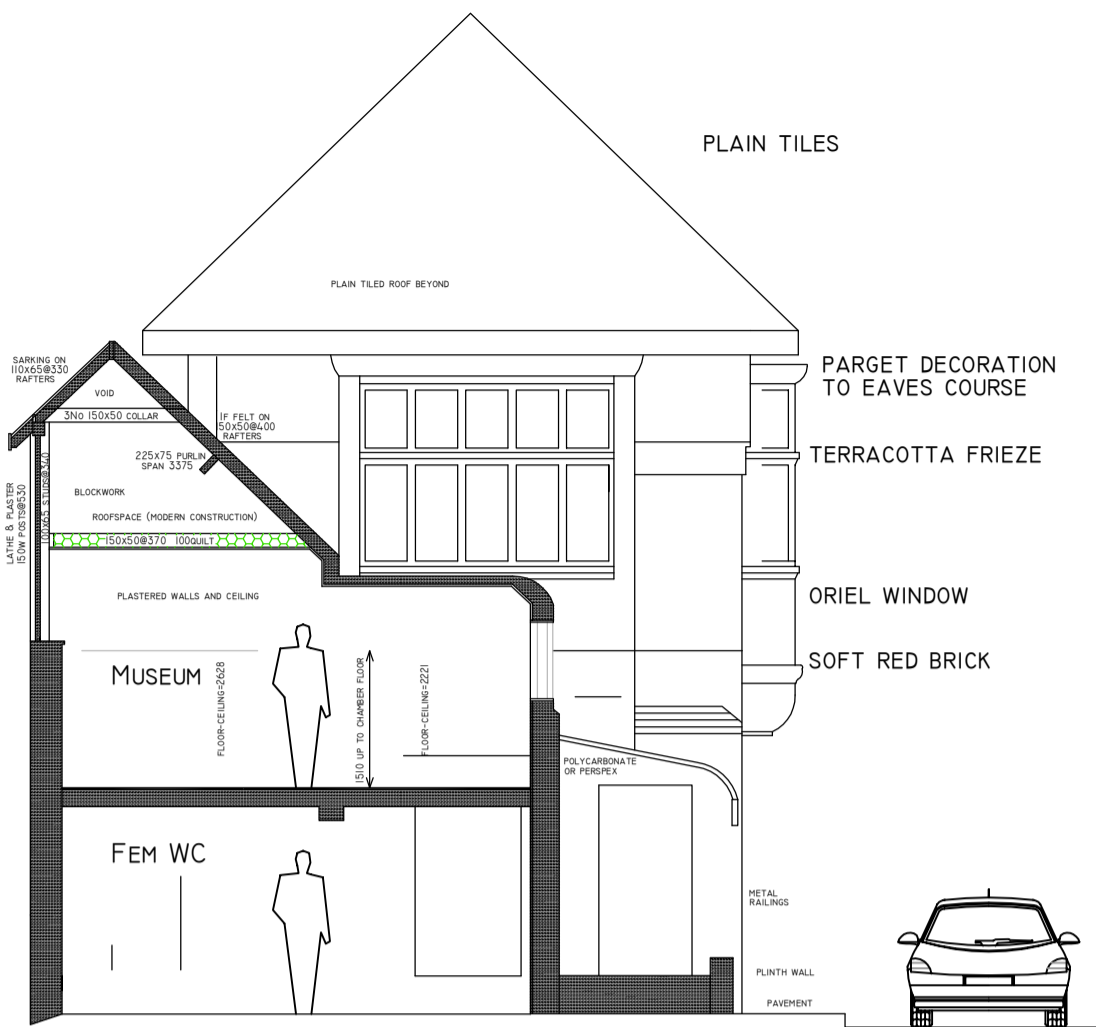
CROSS SECTION EXISTING
