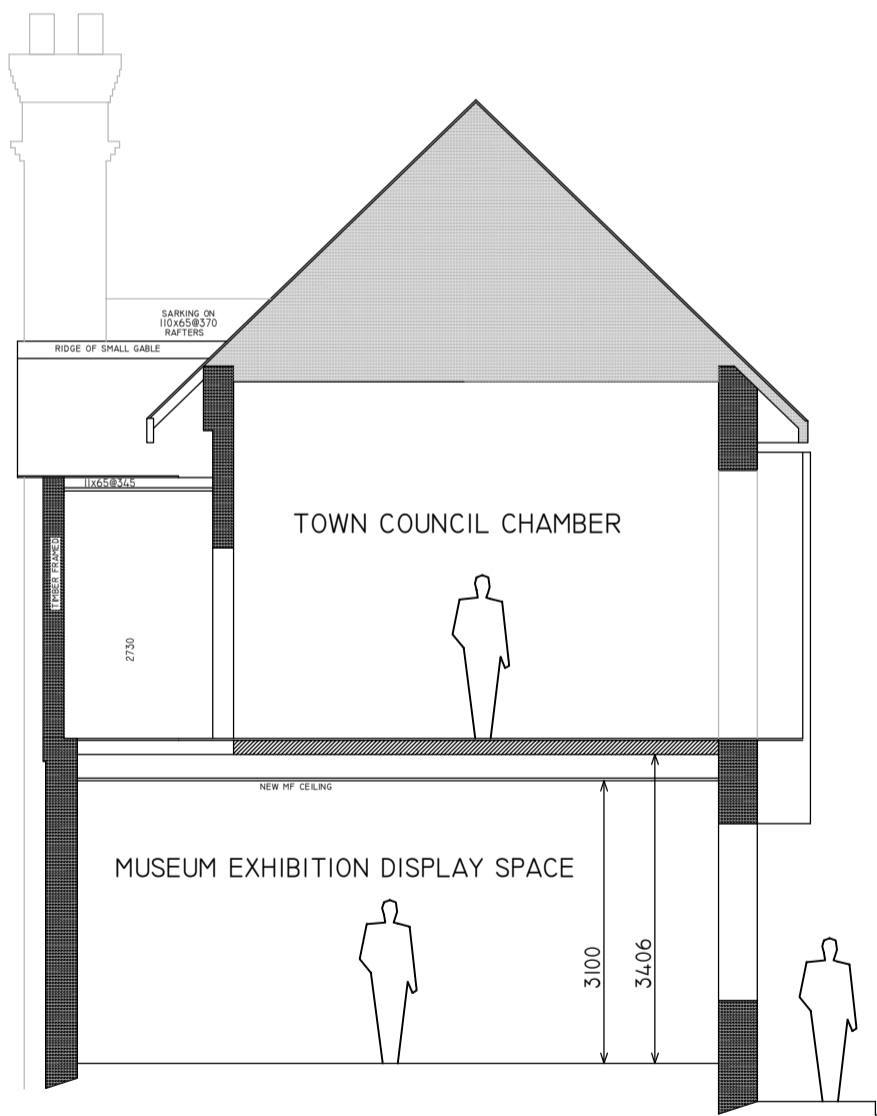
CROSS SECTION PROPOSED
