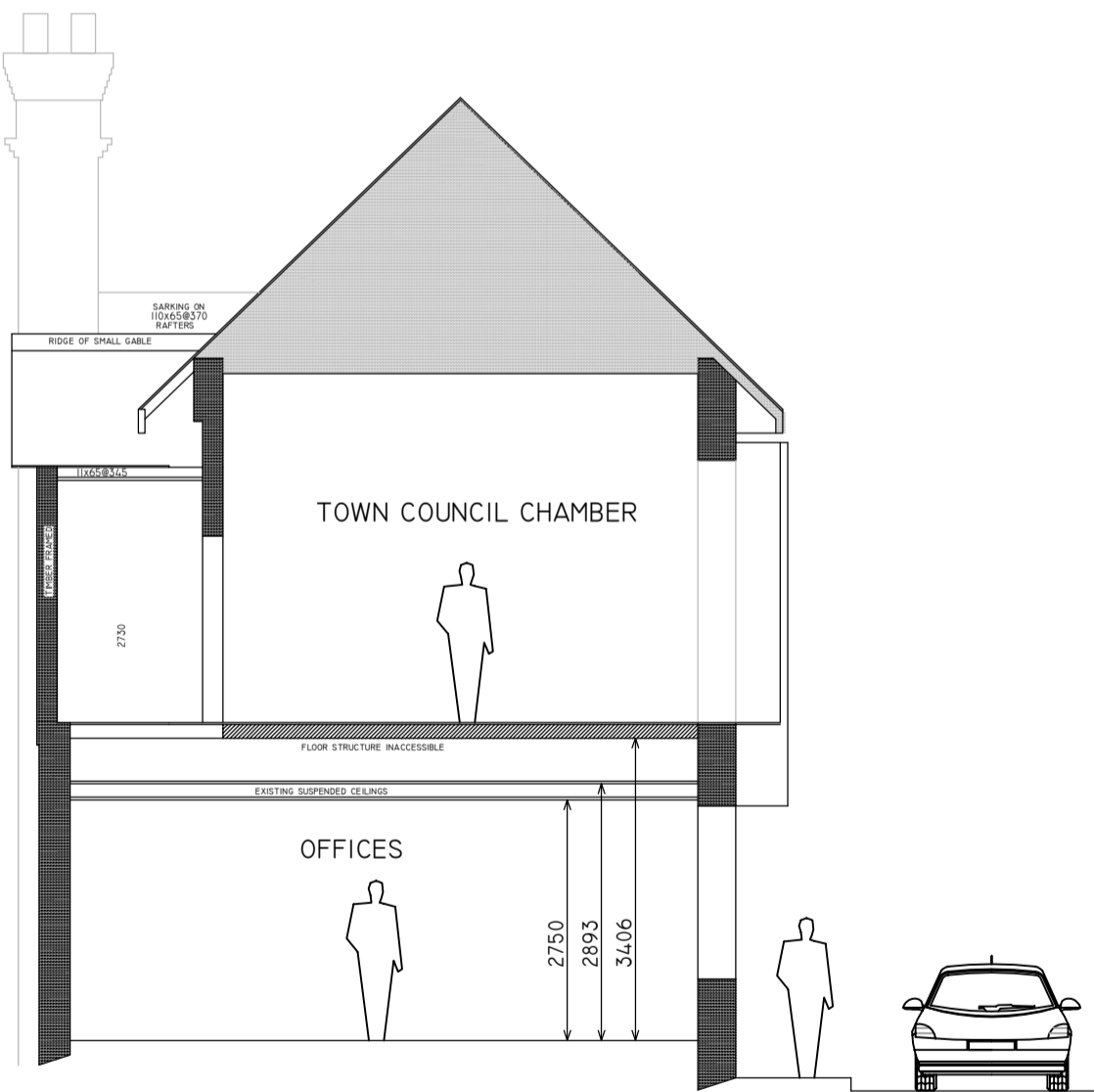
CROSS SECTION EXISTING
